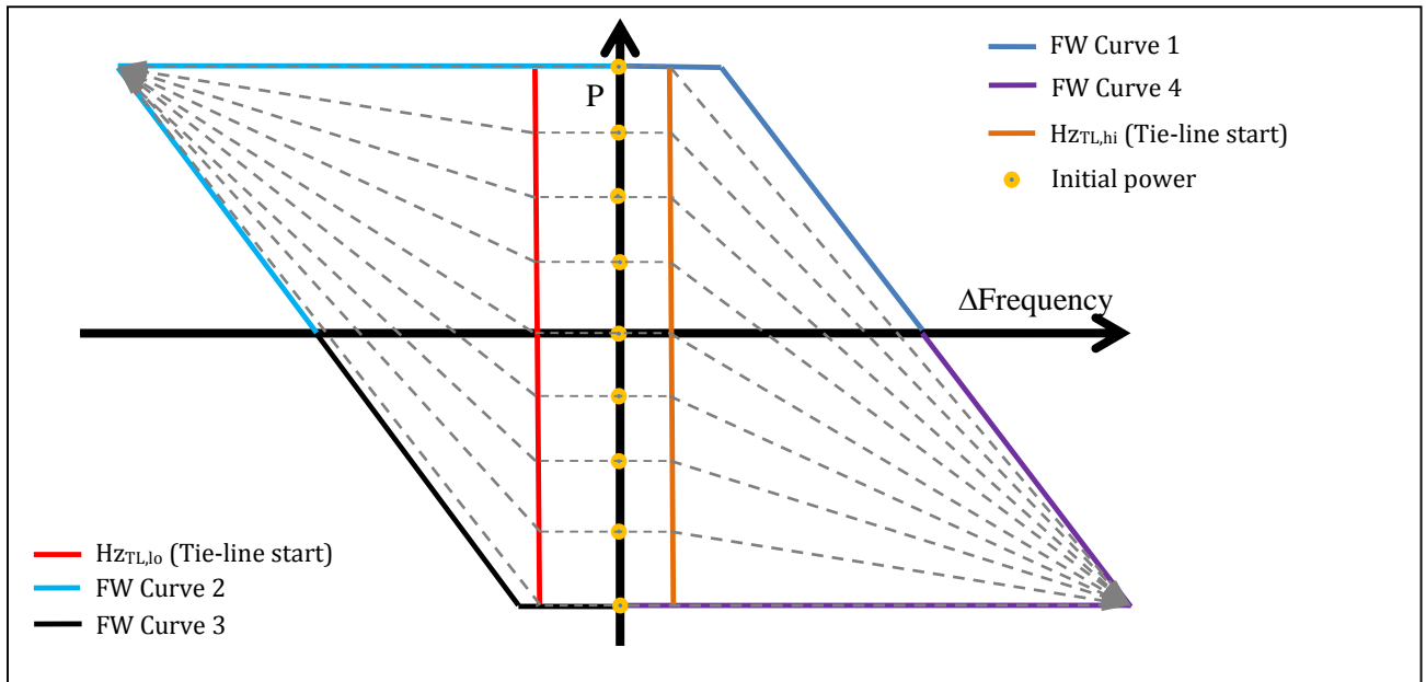
Figure 8. Example FW response with no hysteresis, QuadExit = 1, and TL = 1.
