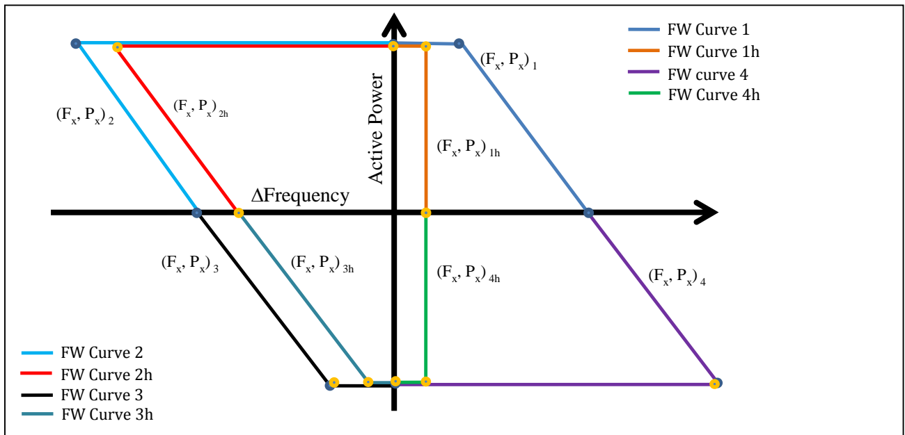
Figure 6. Example FW curves.
