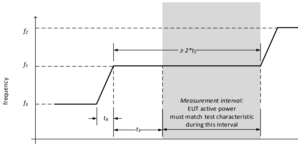
Figure 12. Frequency vs. time during a portion of the frequency-Watt test.
