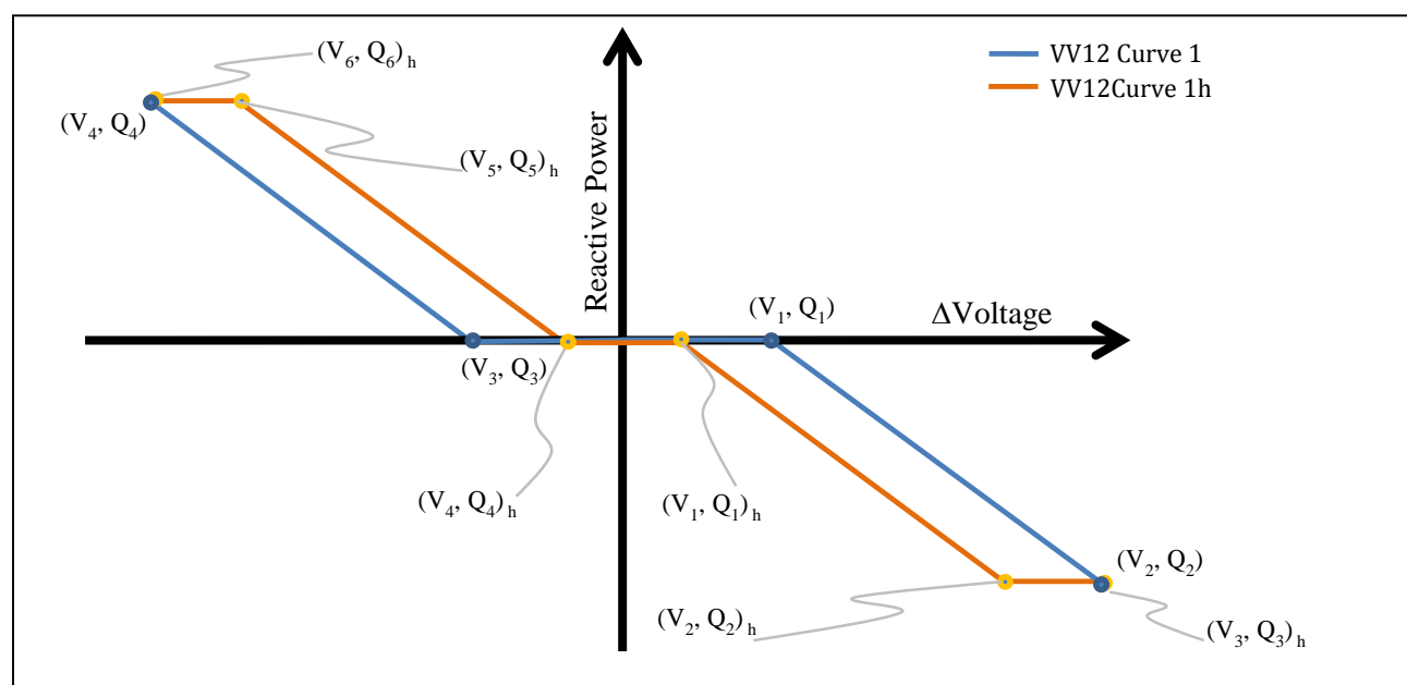
Figure 15. Example VV12 points definition.
