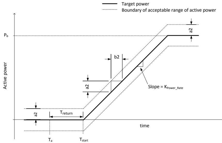
Figure 14. Frequency-Watt test criteria during return to nominal power with hysteresis enabled.
