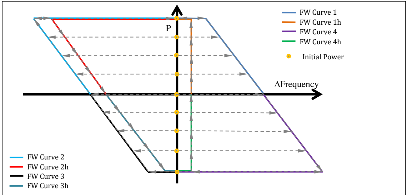
Figure 7. Example FW response with hysteresis, QuadExit = 1, and TL = 0.
