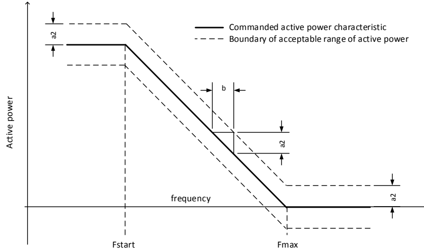
Figure 13. Frequency-Watt test criteria.
