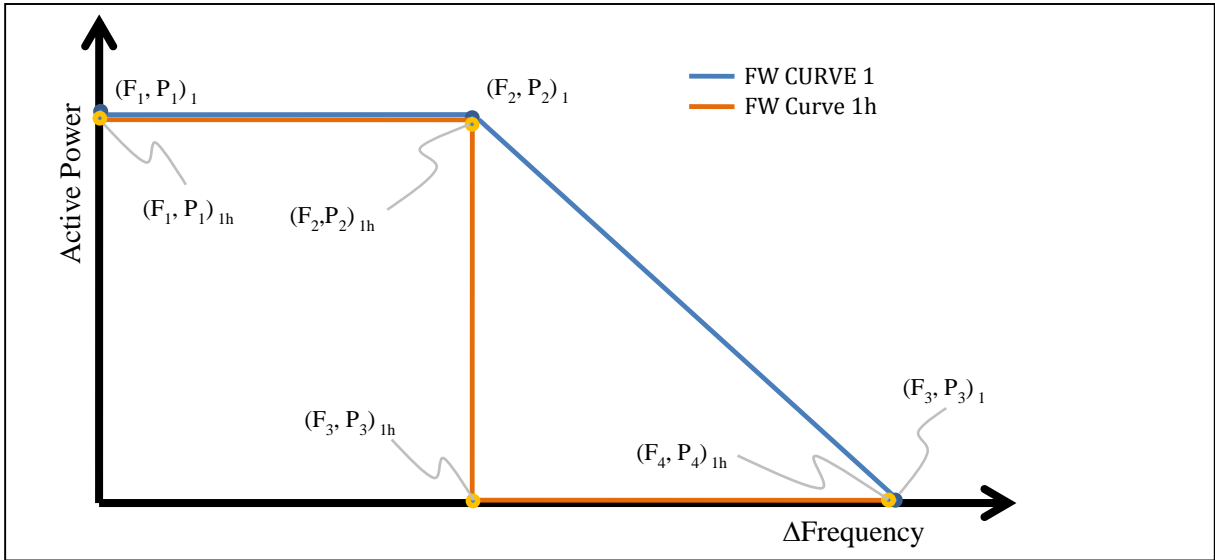
Figure 5. Example FW points definition.
