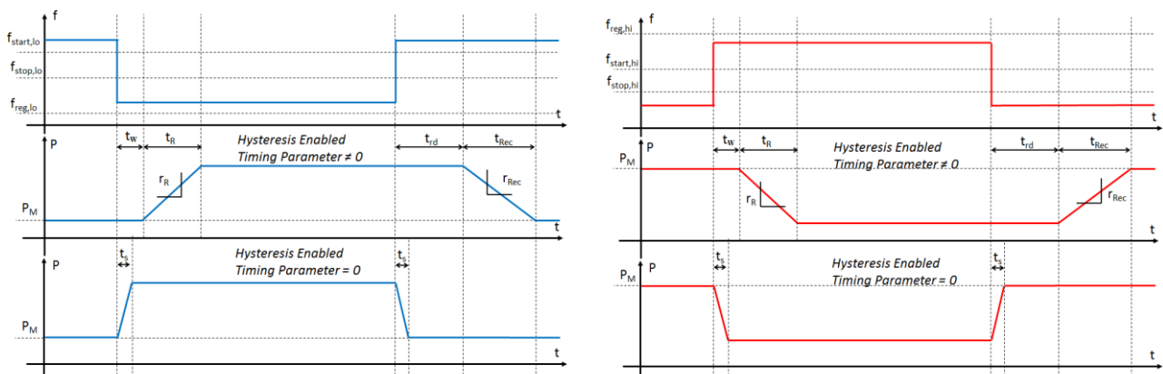
Figure 10. Time domain FW function – Asymmetric Hysteresis Enabled in under-frequency (left side) and in over-frequency (right side).
