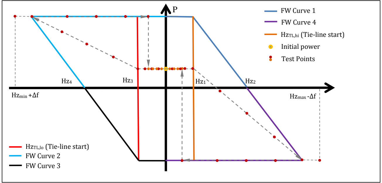
Figure 11. Frequency points required for FW Domain tests.
