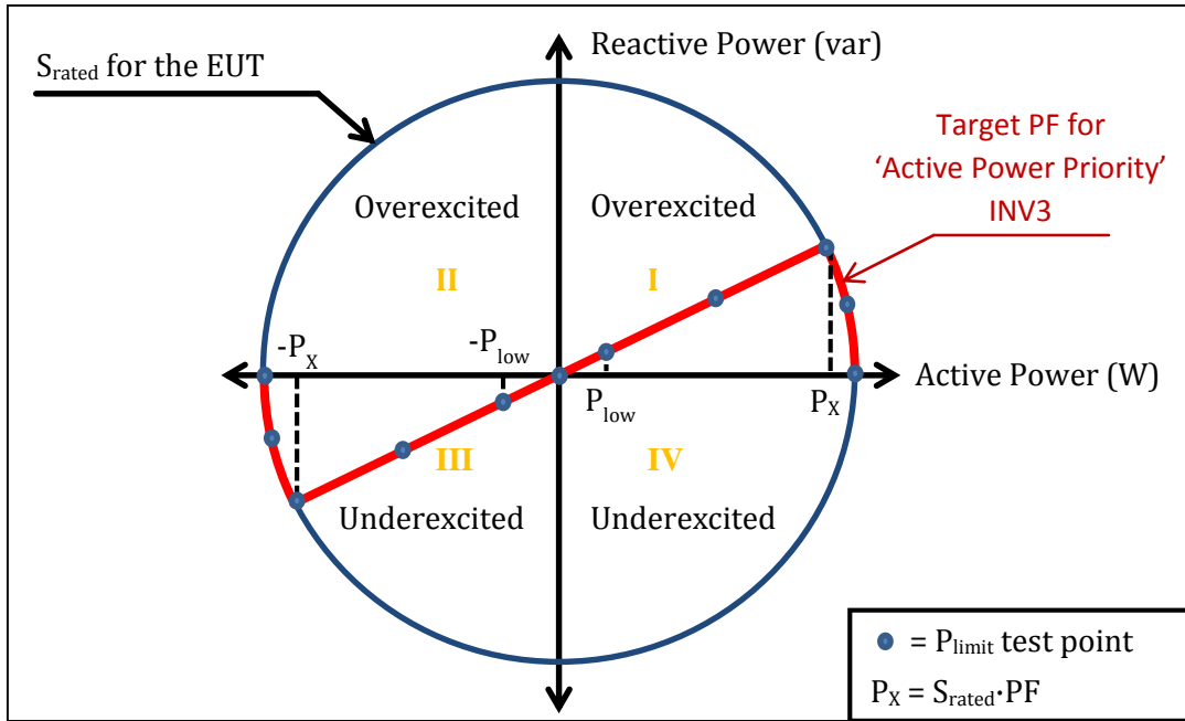
Figure 4. Example target PF for an EUT with 'Active Power Priority' enabled.
