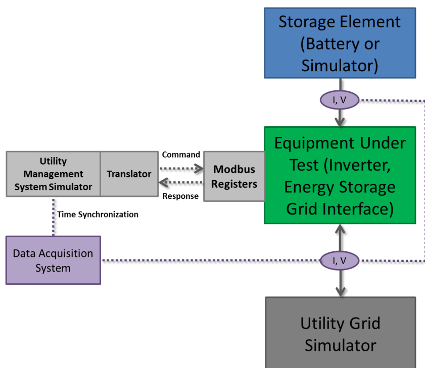
Figure 2. Laboratory setup for energy storage grid support testing.
