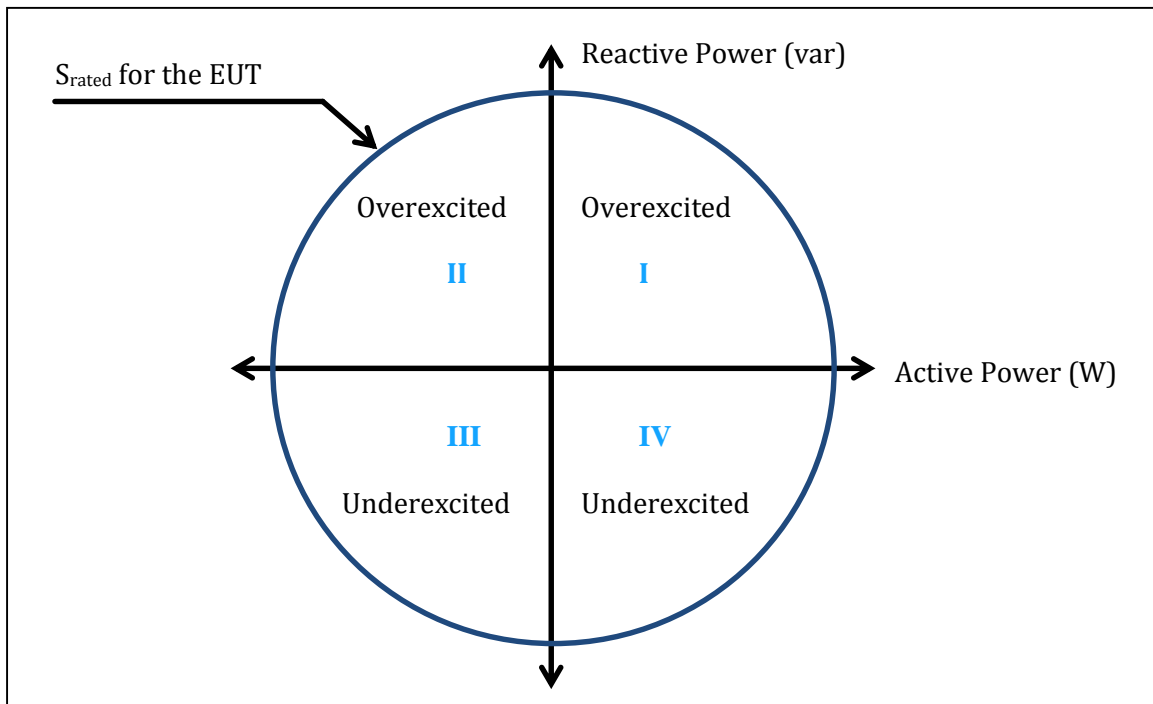
Figure 3. Example EUT P-Q operational limits.
