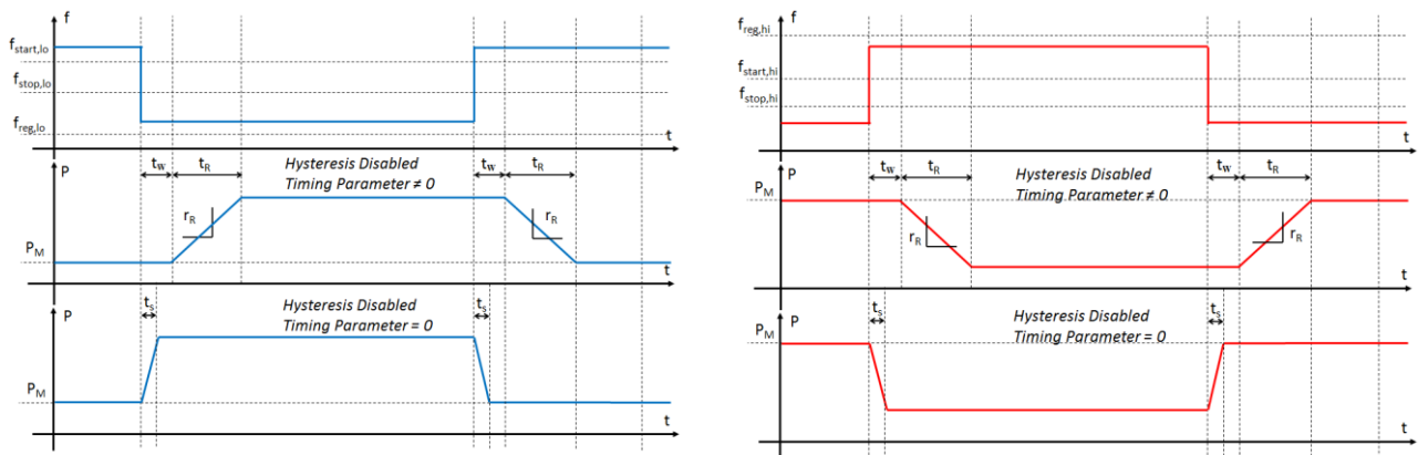
Figure 9. Time domain FW function – Asymmetric Hysteresis Disabled in under-frequency (left side) and in over-frequency (right side).
