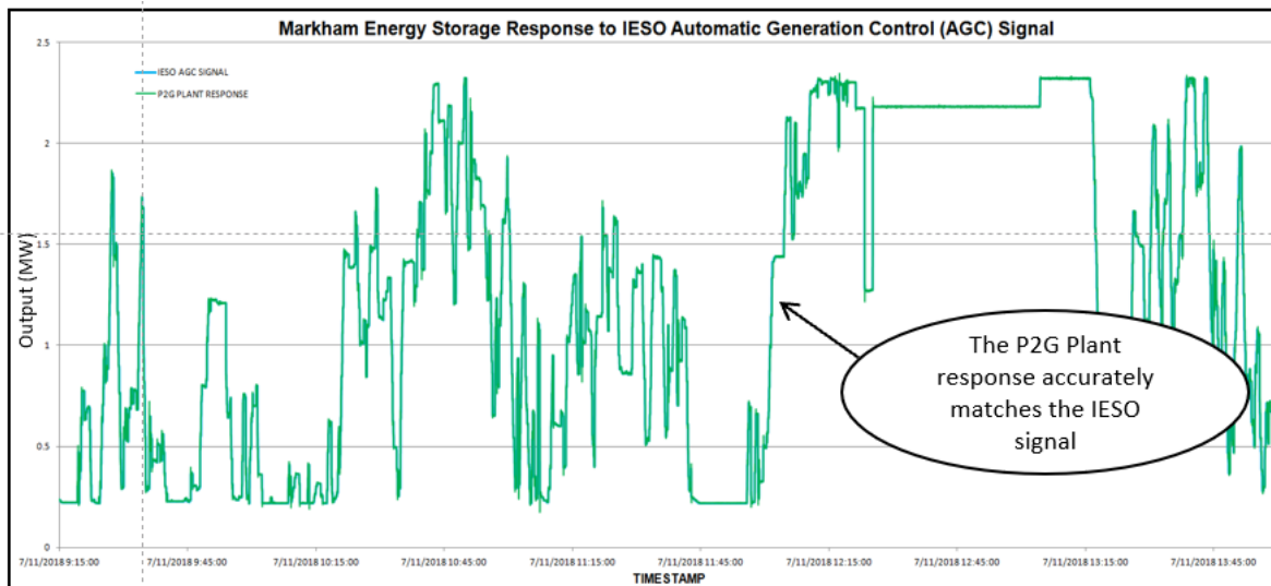
Figure 10: The Power-to-Gas facility output matching the IESO AGC signal exactly on July 11, 2018
