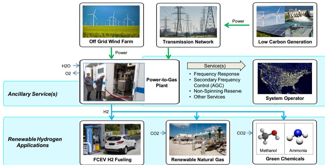
Figure 8: System overview
