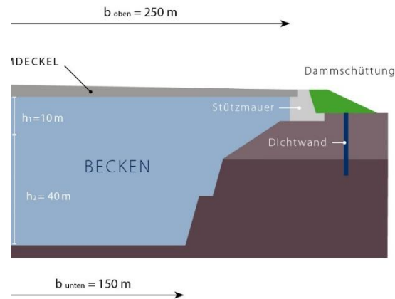
Figure 2: possible construction principle for the seasonal thermal storage
