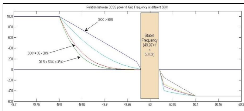
Figure 19: Relation between BESS power & grid frequency at different SOC
