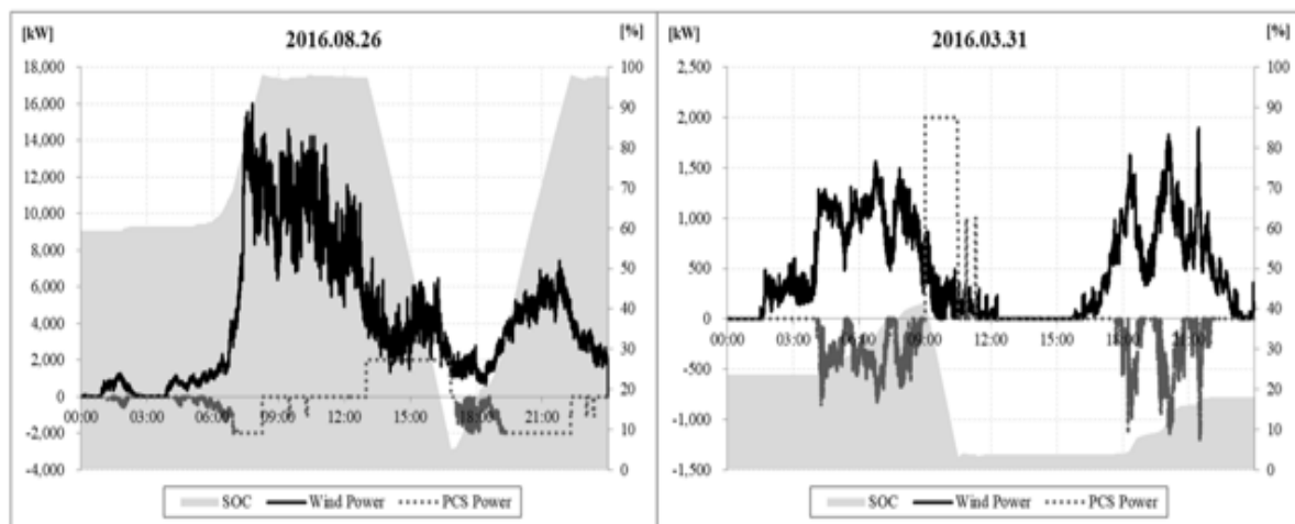
Figure 21: Sampled graphs of daily operation results
