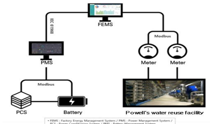
Figure 28: System Configuration
