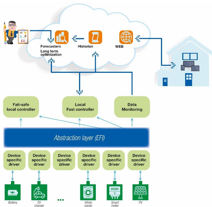
Figure 31: SGSH-architecture
